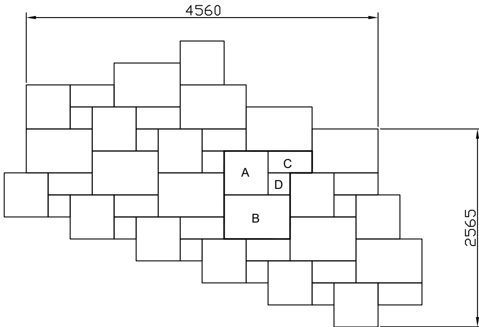
Option 1 - Random Stretcher Course Pattern (8-15mm nominal joint required)
